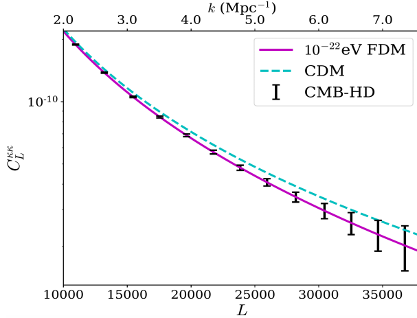
Figure 1: CMB lensing power spectrum for an m \sim 10^{-22} eV FDM model and a CDM model. The error bars correspond to observations with 0.5\mu\text{K} -arcmin CMB noise in temperature and 15 arcsecond resolution over 50% of the sky. Reionization kSZ has also been included as a foreground here. Given these errors, one can distinguish between CDM and a suppression of structure below 10^9 M_\odot with a significance of about 8\sigma .
