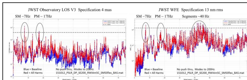
Figure 10: JWST cryogenic Line of Sight and Wavefront Error Performance Predictions [Mosier, Gary, Isolation Requirement, AMTD Report, 2014]
