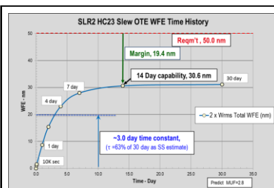
Figure 11: JWST thermal slew [13-JWST-0207 F, 2013]
