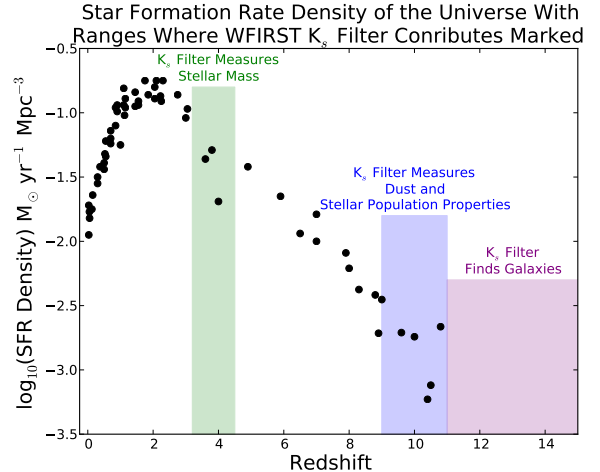
Contributions of WFIRST K_s Filter to Galaxy Evolution Studies
