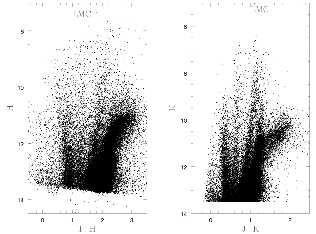
Figure 2. Two versions of the color-magnitude diagram for giant stars in the LMC, one utilizing I - H for the x -axis and one using J - K . The same stars are plotted in the two panels. The J - K diagram clearly sharpens the distinction between different sequences, particularly for carbon stars (the finger pointing up and to the right for J - K > 1.4 , and oxygen rich supergiants (the narrow finger extending above the giant branch, beginning at J - K = 1.2 and K = 10.5 ). The stars plotted are those in the Spitzer SAGE (Meixner et al. 2006) LMC survey; we have cross-matched those stars to the 2MASS and SDSS databases. See Boyer et al. (2011) for a discussion of the post-main sequence demographics that can be distinguished if a K filter is available.
