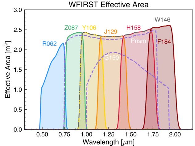
Figure 9. Current baseline WFIRST filter set, showing the effective area at each wavelength. The drop towards the blue within R062 is due primarily to the drop in detector responsivity. By contrast, the detector cutoff at the red end is around 2.5\mu\text{m} .
