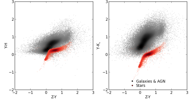
Figure 7. Adding a K_s band to WFIRST (right), increases the separation between stars (red) and other objects (black) compared with the H band (left) allowing for clear differentiation between stars and other objects. Actual data from the COSMOS (Laigle et al. 2016) catalog are shown using HST F814W as a stand in for WFIRST Z band and Ultra-Vista Y, H, and K_s bands. The star/galaxy separation in this plot is based on HST F814W morphology along with the Laigle et al. (2016) catalog.
