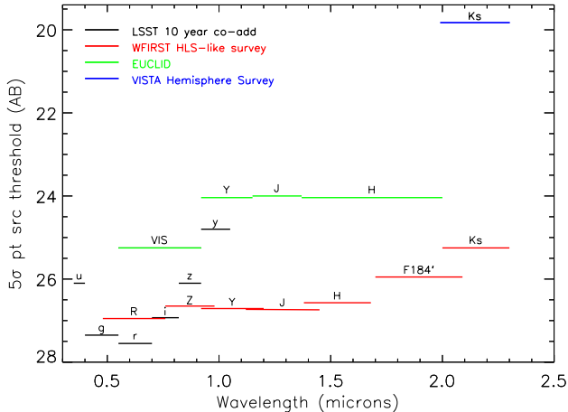
Figure 1. Comparison of the sensitivities of WFIRST, Euclid and LSST, along with VISTA-VHS. The LSST values are for the full 10 year co-add data at the end of the survey. WFIRST limits are for its High Latitude Survey (HLS), or an analogous observing pattern at the other wavelengths, namely R, Z and K_s . We estimated the depths at the latter bands by scaling from the Y, J, H and F184 depths by relative sensitivities. The sensitivity for our proposed K_s filter is shown in the figure based on an assumed telescope temperature of 260 K (the F184 filter sensitivity is also for that assumed temperature).
