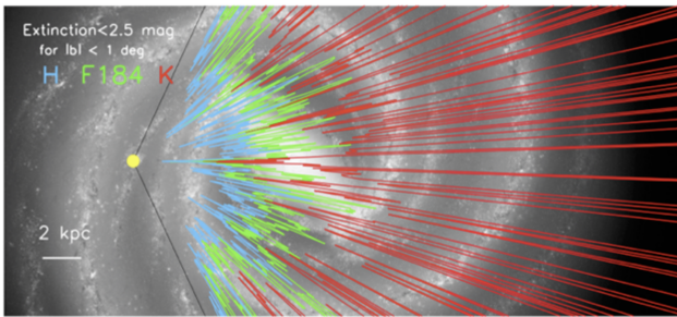
Figure 3. The extinction “horizon” in the H, F184 and K band, i.e. the distance where A_{band} > 2.5 , as a function of Galactic longitude using the three-dimensional dust extinction model of Marshall et al (2006). This map is superimposed on an “artist’s conception” of the Milky Way Galaxy by Robert Hurt. At each longitude slice, the length of the lines represent the distance corresponding to the maximum extinction at that wavelength for any latitude value. Note the volume of the Galaxy with modest (less than a factor of ten) extinction expands dramatically by going to the K band. Going to the K-band allows us to probe directly the farthest reaches of the galaxy and map the outer spiral arms.
