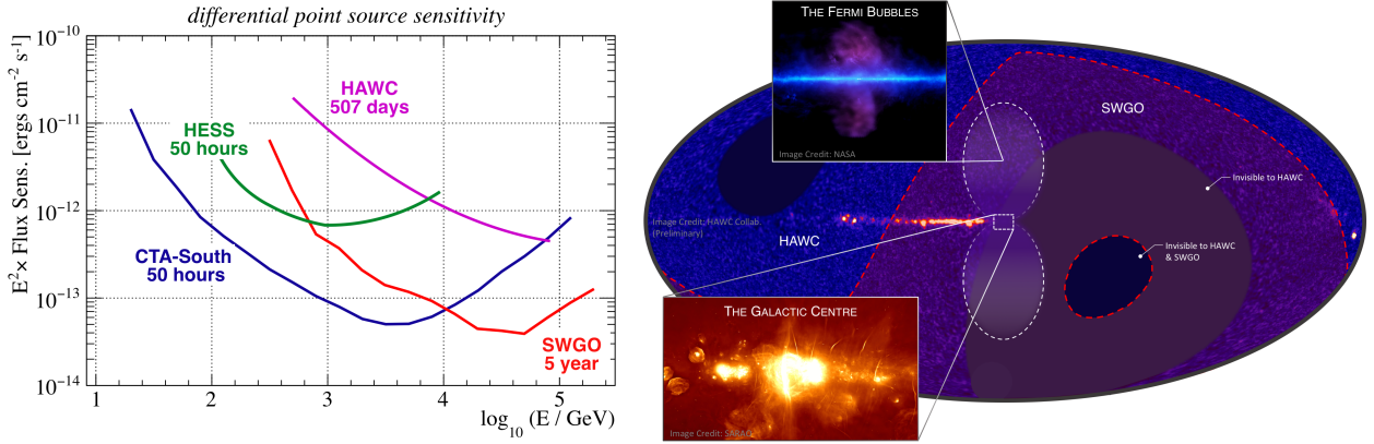
Figure 1: Left : Differential point-source sensitivity as a function of energy for the proposed SWGO detector compared to other existing or proposed instruments. Right : Sky coverage of SWGO in Galactic coordinates overlaid on HAWC significance map containing over 50 sources.
