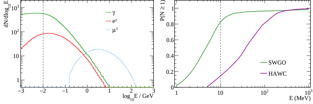
Figure 3: Left : Average number density at 5 km above sea level for air showers initiated by 1 TeV protons (adapted from [91]). Right : Detection threshold probability for secondary gamma rays of the SWGO unit design. The top compartment is compared to a HAWC detector unit. A 8" PMT R5912 Hamamatsu PMT has been assumed in this simulation. The vertical dashed line in both panels indicates 10 MeV.
