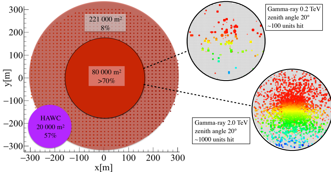
Figure 4: Left : Array configuration with instrumented areas and ground coverage indicated (and HAWC equivalent for comparison). Right : SWGO response for two simulated gamma-ray events. The color coding indicates the time gradient. The 200 GeV example illustrates the large particle spread even at low energy.
