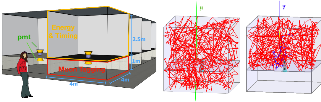
Figure 2: Left: Illustration of detection unit design. Right: Muon and gamma-ray passing through a detection unit. Red lines indicate a fraction of the Cherenkov photon tracks, while the green, blue, and yellow lines indicate the tracks of muons, gamma rays and electrons respectively.
