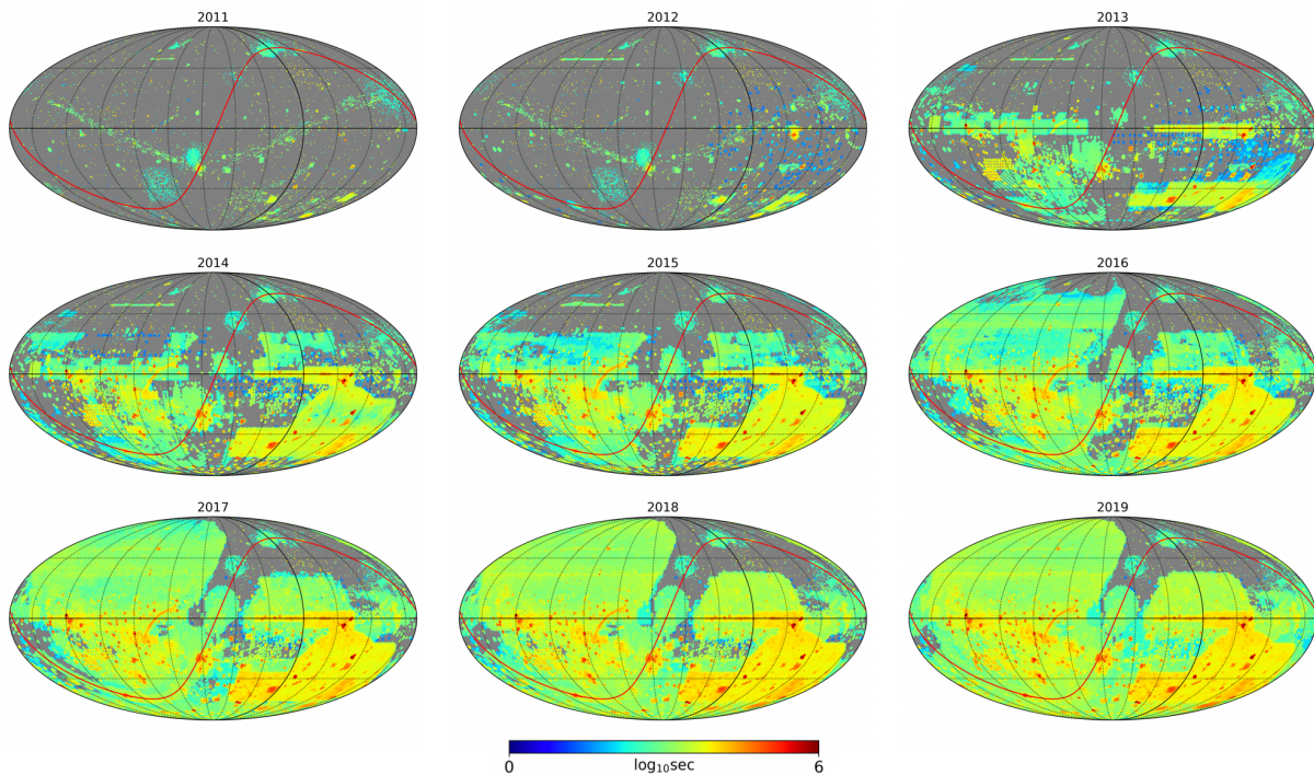
Figure 1: Sky map of integrated exposure time of NOAO archival data holdings (evolution from 2011 to 2019.)
