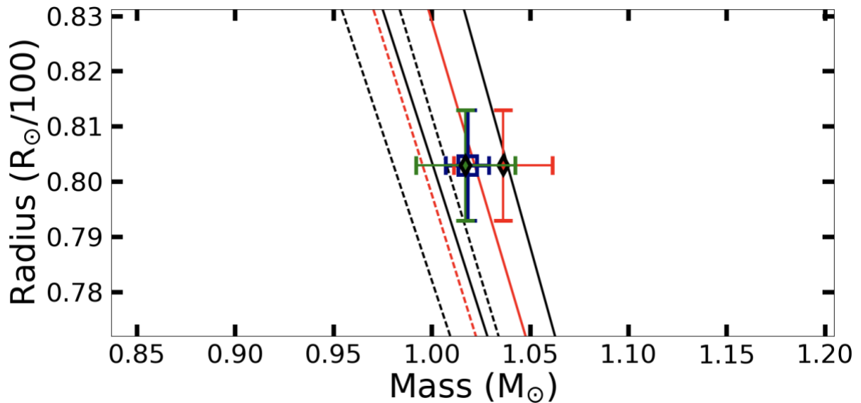
Figure 1. Mass and radius of Sirius B measured from the gravitational red-shift (red and green diamonds, corresponding to two slit positions in the STIS spectrograph) compared to the dynamical values (blue square). Solid and dashed lines represent theoretical mass-radius relations for thick and thin H-layers respectively (Red lines - T_{\text{eff}} = 25,922\text{K} for Sirius B, black either side for 10,000K and 40,000K).
