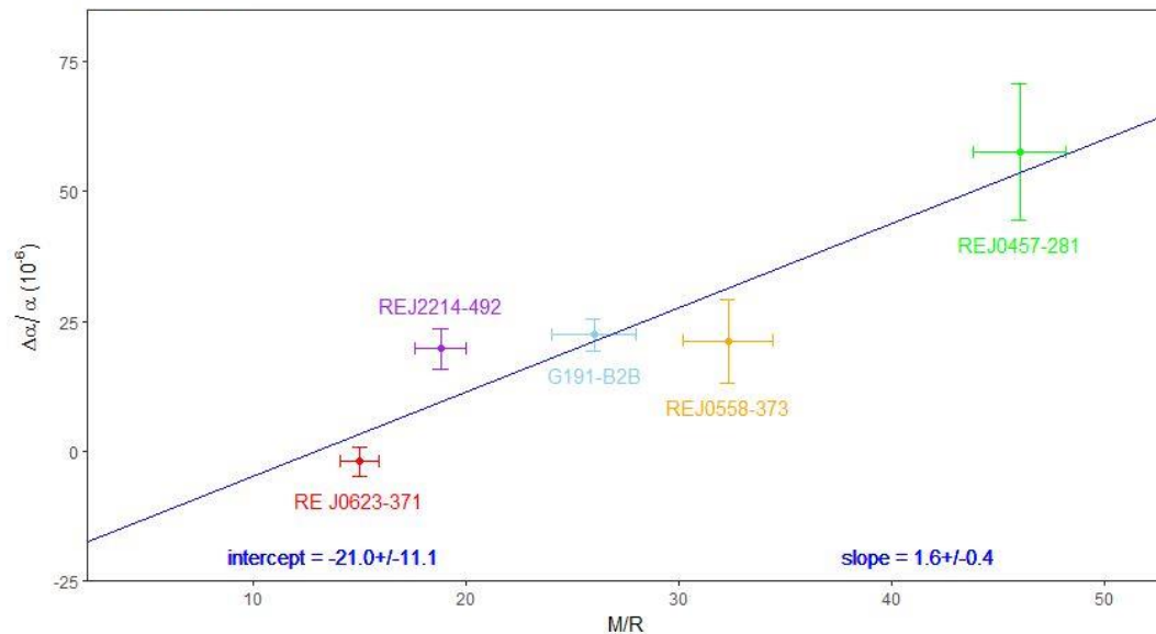
Figure 2. Limits on the variation of the fine structure constant as a function of “compactness” (M/R) for five hot H-rich DA white dwarfs, obtained through UV spectroscopy with HST.
