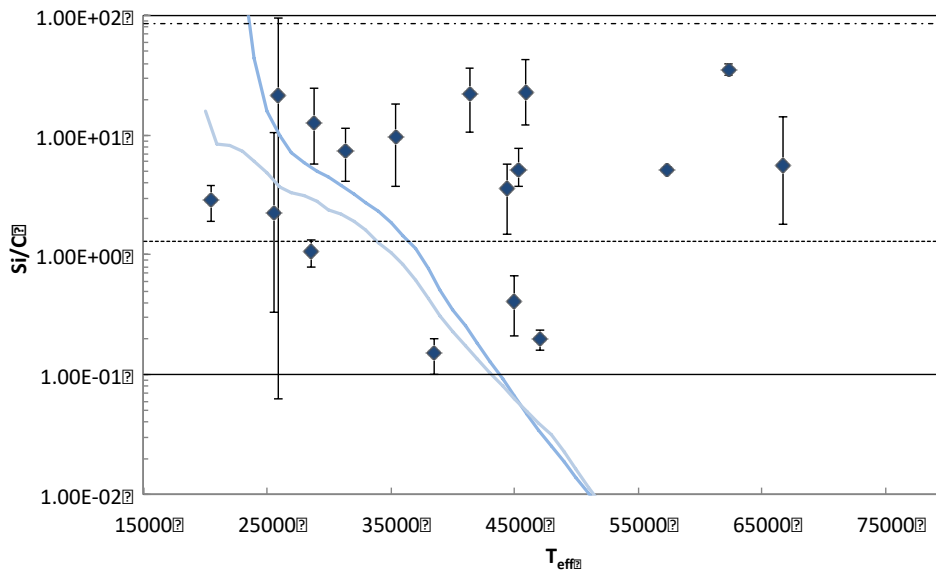
Figure 3. Si to C ratio for a sample of 17 white dwarfs observed in the far UV by FUSE. Most stars show evidence for accretion of rocky material (solid line – solar abundance, dotted line – CI chondrite, dot-dash line – bulk Earth).
