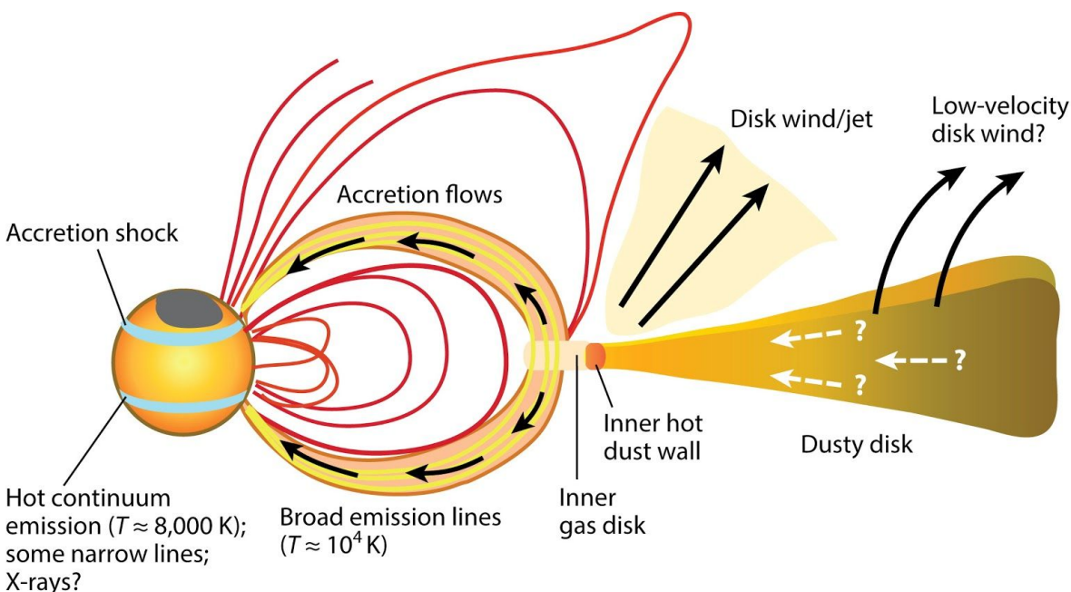
Fig. 1: Disk accretion cartoon, reproduced with permission (Hartmann, Herczeg, & Calvet 2016).
