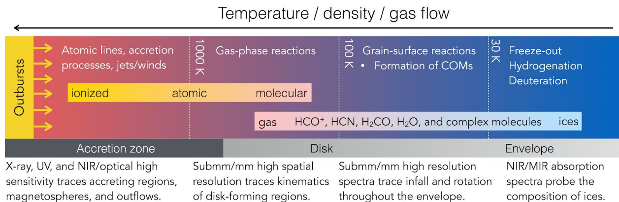
Fig. 2: Representative chemical and kinematic zones in protostars (courtesy: Y.-L. Yang).
