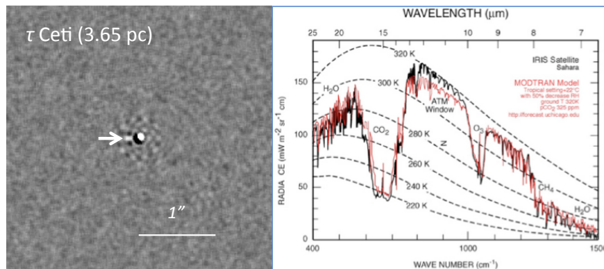
Figure 2: Thermal infrared ( 10 \mu\text{m} ) imaging and characterization. Left: Simulated image of RV candidate \tau Ceti e ( 1.3 R_{\text{Earth}} planet at 0.5 AU, as marked) in equilibrium with the host star at the inner edge of the “habitable zone”. Scale bar is 1'' for reference. A coronagraph and advanced post-processing techniques are used to suppress the central star. Right: Observed and modeled spectrum of Earth at 7-13 \mu\text{m} showing major absorption features due to atmospheric constituents.
