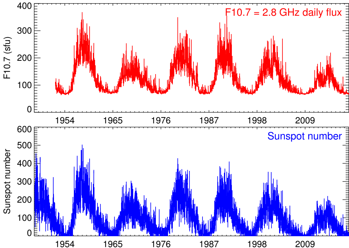
Figure 1: Plots of daily values for sunspot number (lower panel) and the solar radio flux at a wavelength of 10.7 cm (2.8 GHz), known as F10.7 (upper panel) over the past 7 decades.
