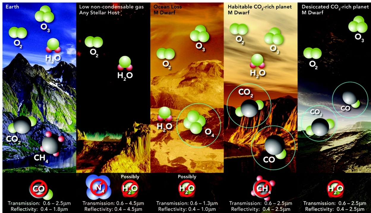
Figure 2: Possible O 2 and O 3 biosignature false positives. Top panels show atmospheric constituents. Circled gases show false positive indicators. Bottom panels indicate species that should be absent for a given false positive to apply. Only one scenario plausibly applies to Sun-like stars for planets with low non-condensable gas inventories (i.e. low-pressure atmospheres), but such a planet could be identified given constraints on total atmospheric pressure. This may be possible with sufficient signal-to-noise observations (Feng et al. 2018; discussion in T. Robinson whitepaper). Figure credit: Meadows (2017).
