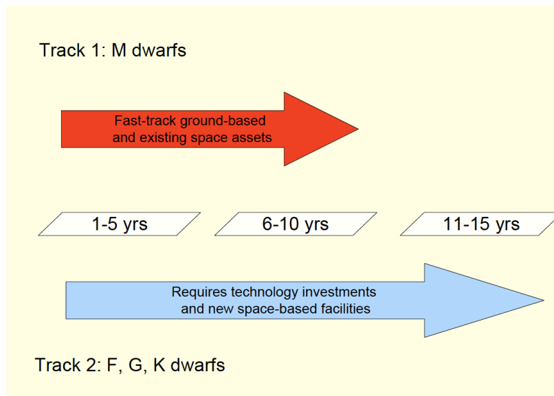
Figure 1: The recommended exoplanet science strategy from the 2008 Report of the ExoPlanet Task Force . Track 1 (M dwarfs) is now in progress. Track 2 (F, G, K dwarfs; i.e. “Sun-like” stars) will require major new technology and facilities for significant progress. Figure credit: Figure 1 from the Report of the ExoPlanet Task Force (Lunine et al., 2008).
