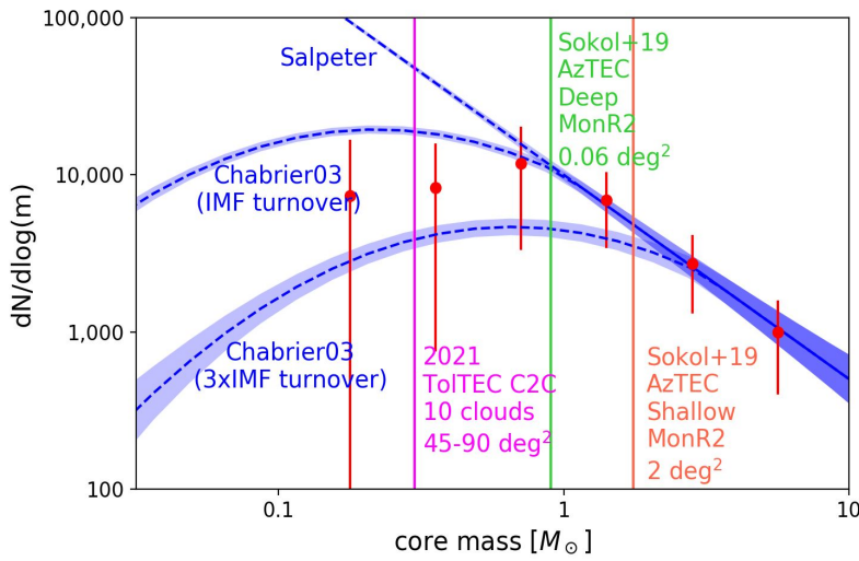
Figure 2: Core mass functions, present and future. Sokol et al. (2019) CMF for the MonR2 cloud is shown in red points (scaled up by 10x to match models) with three sigma error bars. Large statistical uncertainties and limited depth result in weak constraint on the low-mass end of the CMF. Predicted CMFs (Salpeter 1955, Chabrier 2003) scaled to the size of a planned large survey of ten nearby giant molecular clouds, the ToI TEC Clouds to Cores (C2C) Public Legacy Survey, are plotted in blue. Survey completeness limits (90%) for the Sokol et al. (2019) and ToI TEC C2C surveys are red, green and magenta vertical lines, respectively.
