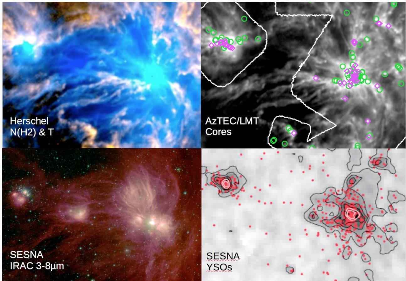
Figure 1: A demonstration of the complex ecosystem of an active molecular cloud (MonR2, here as an example), with pre-stellar and protostellar cores and other YSOs forming co-spatially. Upper left: Herschel greybody fits reveal the wide range of gas column densities (intensity) and spatial variance in dust temperature (color, with red for T < 10\text{K} and blue for T > 20\text{K} ) caused by stellar feedback (Pokhrel et al. 2016). Upper right: Herschel column density in greyscale, overlaid with starless (green) and protostellar (magenta) core positions (Sokol et al. 2019). Lower left: Spitzer Extended Solar Neighborhood Archive (SESNA) 3-8 micron image of the same field of view, revealing UV-excited PAH-emission-traced bubble features (Gutermuth et al. 2011; Gutermuth et al. in prep.). Lower right: 2MASS-derived near-IR extinction map overlaid with A_v contours (black/white lines) and IR-excess-bearing YSO positions in red (Gutermuth et al. 2011).
