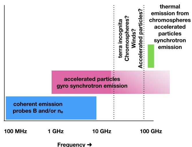
Figure 2: Schematic diagram of the radio-mm-sub-mm spectral region and the types of fundamental information on stellar atmospheres that can be returned from studies of these different areas.
